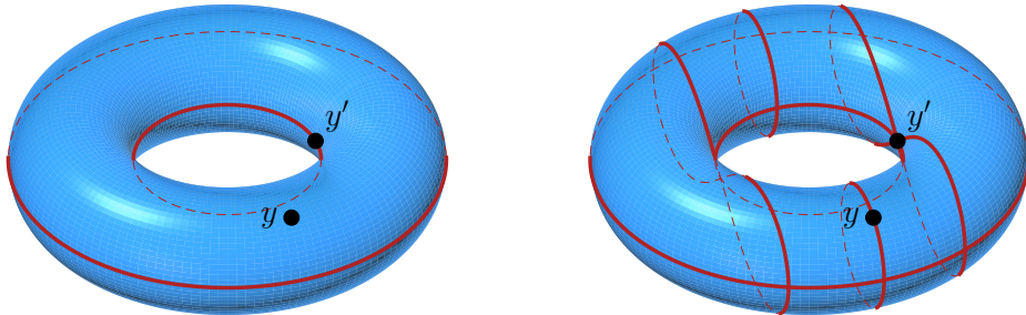
Figure 5.1. Illustration of the two steps of Canny’s algorithm on a torus in \mathbf{R}^3 , with two query points \mathbf{y} and \mathbf{y}' . On the left, the one-dimensional polar variety associated with the projection on the plane below is computed. It intersects the unique connected component, but this intersection is not connected, and does not contain neither \mathbf{y} nor \mathbf{y}' . To repair these failures, we add fibers containing the critical points of a projection on a line and the query points. This gives the right figure.
