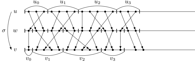
Fig. 3. Double Factorization
