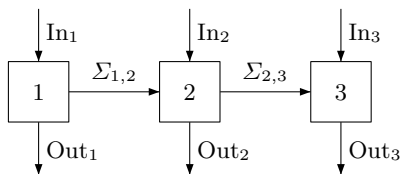
Fig. 1. An architecture
