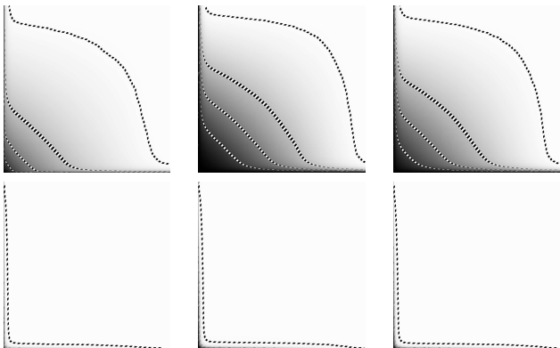
Fig. 16. Dense ER graph: clustering, number of triangles, and number of triples. k = 100 , N = 10^4 , USP (first row) and ASP (second row).
