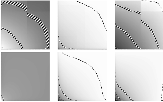
Fig. 23. Clustering, number of triangles, number of triples for the core of the original Mercator graph (first row) and a GL graph with the same distribution of cliques sizes (second row). USP explorations.
