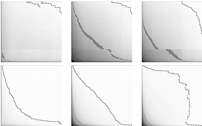
Fig. 24. Clustering, number of triangles, number of triples for the original nec graph (first row) and a GL graph with the same distribution of cliques sizes (second row). USP explorations.
