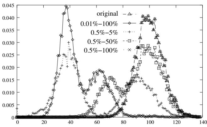
Fig. 12. ER graph: degree distribution. k = 100 , N = 10^4 , ASP.
