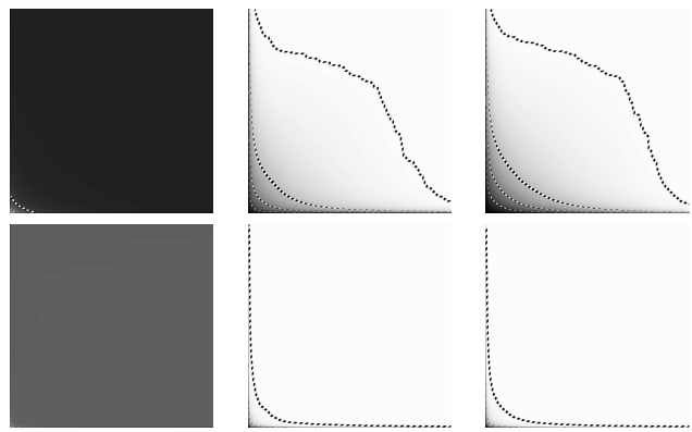
Fig. 17. AB graph: clustering, number of triangles, and number of triples. k = 10 , N = 10^4 , USP (first row) and ASP (second row).
