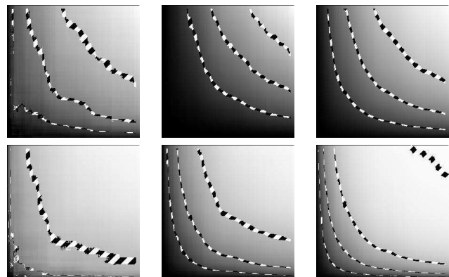
Fig. 26. Clustering, number of triangles and triples for the nec graph using random sources and destinations and shortest-paths. USP (first row) and ASP (second row).
