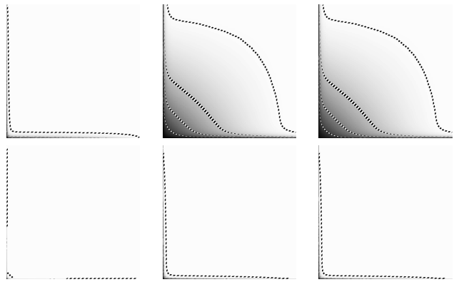
Fig. 3. ER graph: number of nodes, number of links, and average degree. k = 100 , N = 10^4 , USP (first row) and ASP (second row).
