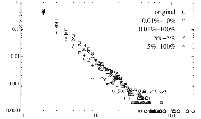
Fig. 14. DM graph: degree distribution. N = 10^4 , USP (top) and ASP (bottom).
