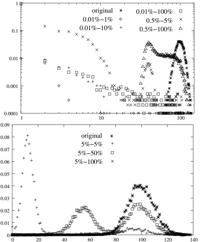
Fig. 11. ER graph: degree distribution. k = 100 , N = 10^4 , small number of sources (top log-log scale) and large number of sources (bottom normal scale). USP
