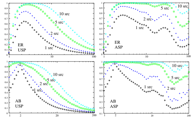
Fig. 1. Proportion of discovered links versus average degree in an ER graph (first row) and in an AB graph (second row) when one uses a USP exploration (left column) or an ASP one (right column). Plots are given for various (small) numbers of sources (namely 1, 2, 5 and 10). All the nodes are taken as destinations. N = 10^4 .
