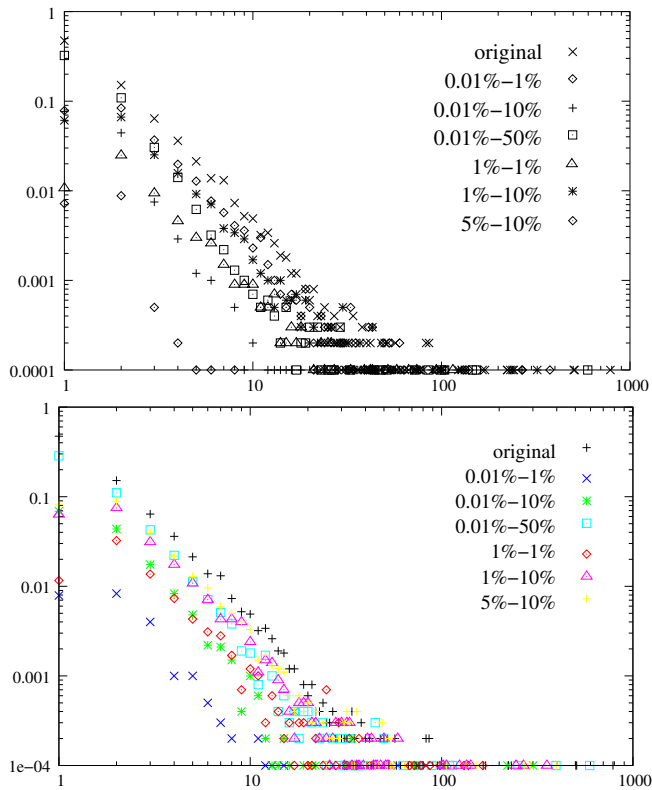
Fig. 13. MR graph: degree distribution. \alpha = 2.5 , N = 10^4 , USP (top) and ASP (bottom).
