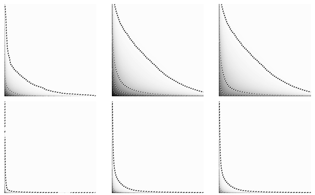
Fig. 5. AB graph: number of nodes, number of links, and average degree. k = 10 , N = 10^4 , USP (first row) and ASP (second row).
