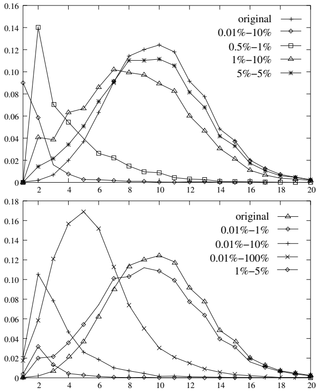
Fig. 10. ER graph: degree distribution. k = 10 , N = 10^4 , USP (top) and ASP (bottom).
