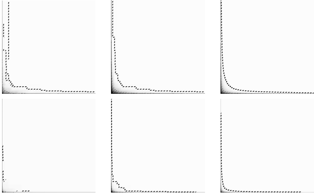
Fig. 15. ER graph: clustering, number of triangles, and number of triples. k = 10 , N = 10^4 , USP (first row) and ASP (second row).
